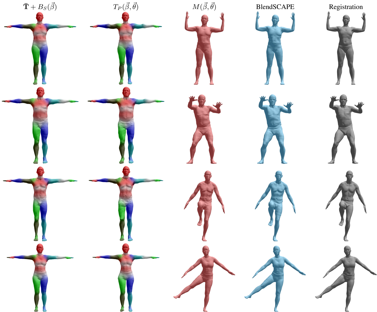
Figure 10: Model fitting with intermediate stages. We fit both BlendSCAPE (blue) and SMPL-LBS, M(\vec{\beta}, \vec{\theta}) , (red) to registered meshes by optimizing pose and shape. \bar{T} + B_S(\vec{\beta}) shows the estimated body shape and T_P(\vec{\beta}, \vec{\theta}) shows the effects of pose-dependent blend shapes. Here we show SMPL-LBS, because T_P shows more variation due to pose than SMPL-DQBS.
